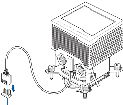
4-pin CPU_FAN header or W_PUMP+ header
